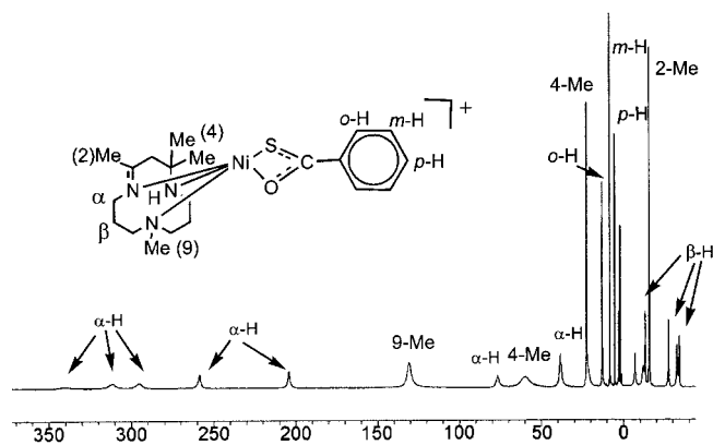
Figure 7. 1 H NMR spectra [in (CD 3 ) 2 CO solution at room temperature] of complex 12 .
